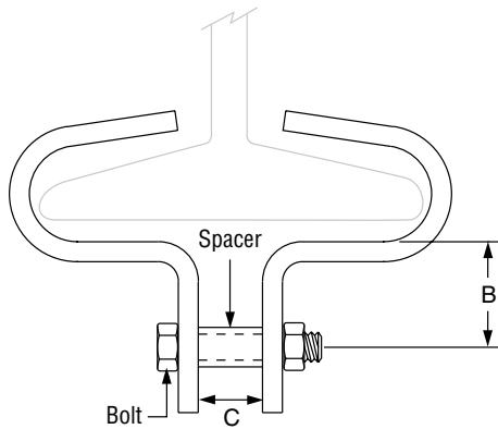
FIG. 134: DIMENSIONS (IN) • LOADS (LBS)
