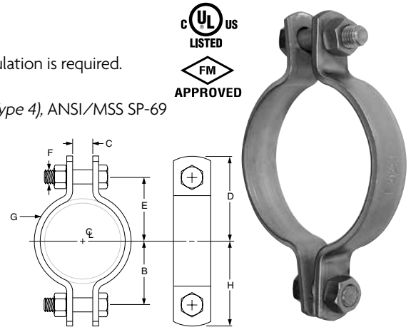
Note: This picture is representative of a typical Figure 212. Distance between clamp ears beneath pipe may or may not be equal to upper gap.
